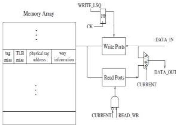
FIG.3. Information Buffer
