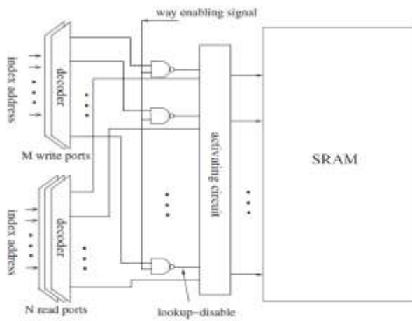
FIG.2. Architecture of LSQ Tag Array
